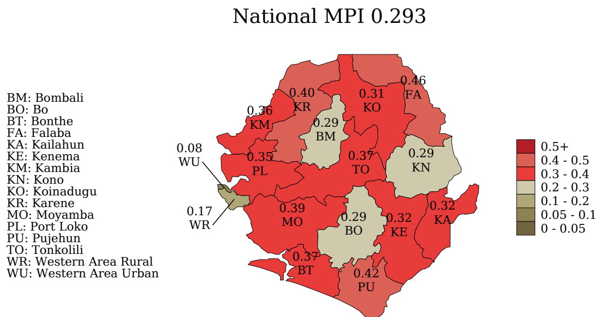
Figure 9. Mapping MPI Value by Subnational Region
