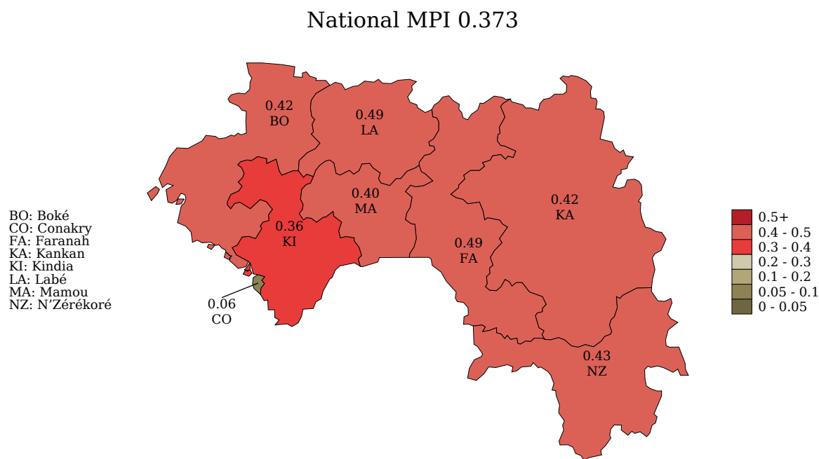
Figure 9. Mapping MPI Value by Subnational Region
