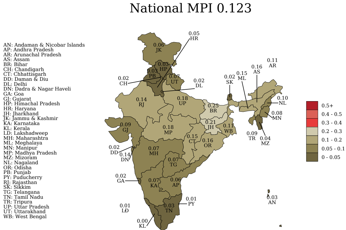
Figure 9. Mapping MPI Value by Subnational Region
